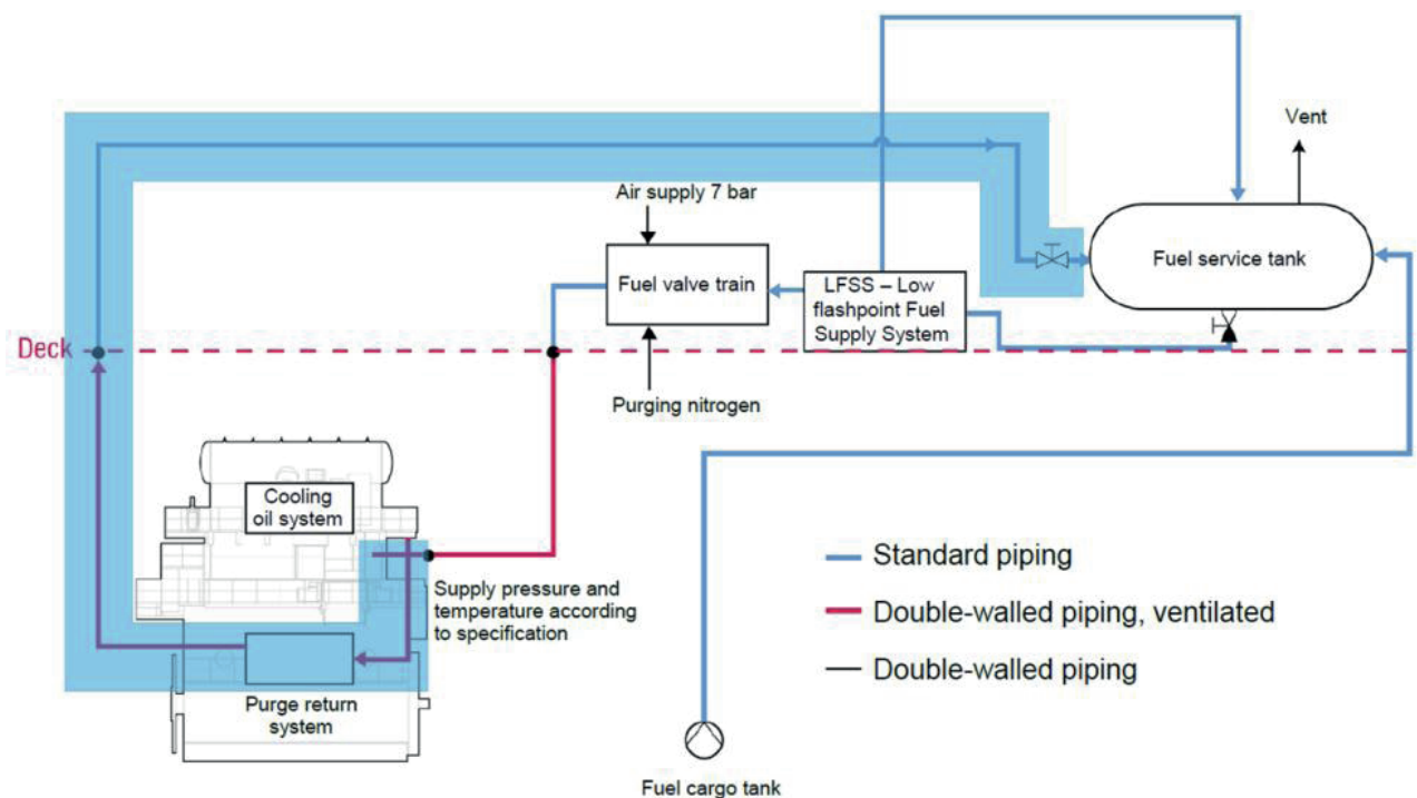
Figure 5-5: Handling and processing of methanol after the main engine /20/
