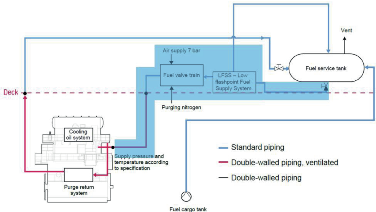
Figure 5-3: Handling and processing of methanol towards the main engine 20/
