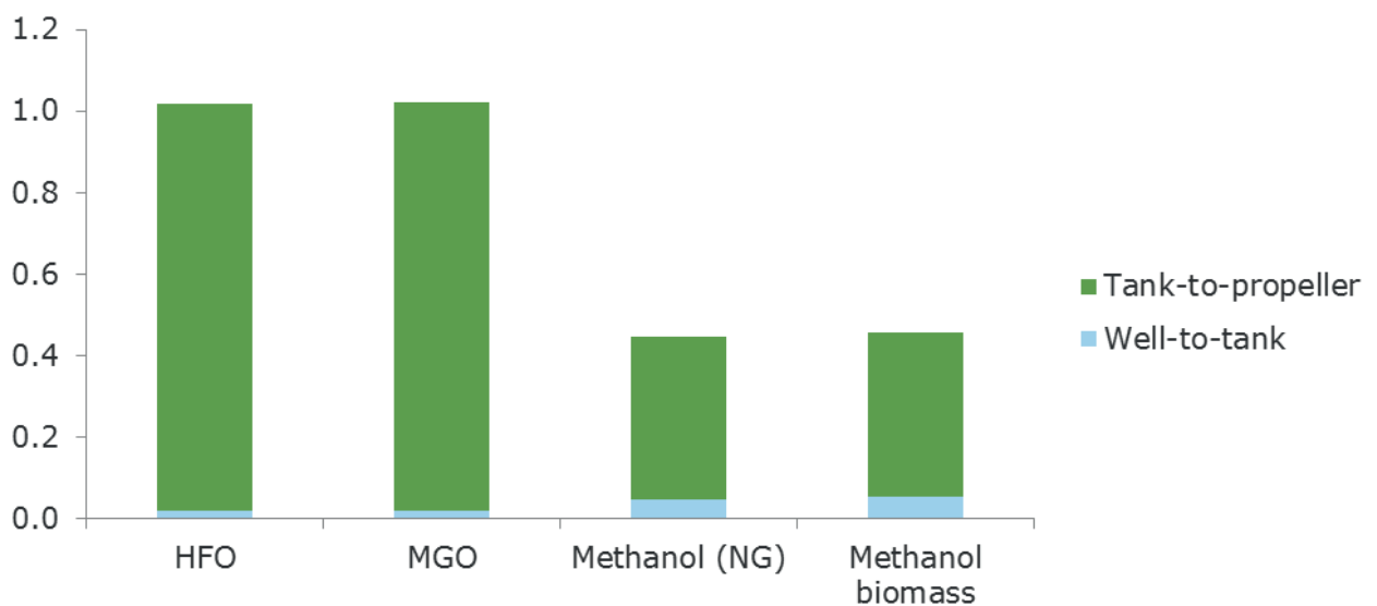
Figure 4-10: Lifecycle emissions of NO x from methanol compared to conventional fuels
