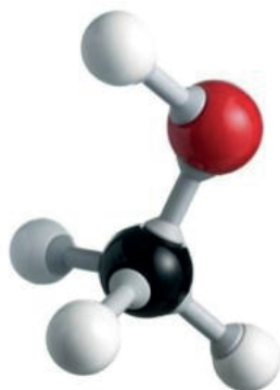
Figure 2-1: Symbolic representation of methanol molecule, CH 3 OH
